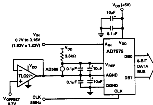
Figure 2. AD7575 AGND Bias Scheme
