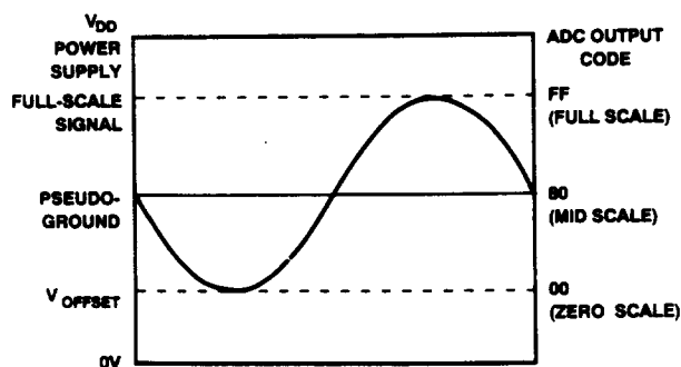
Figure 1. Pseudo-Ground Biasing Arrangement
